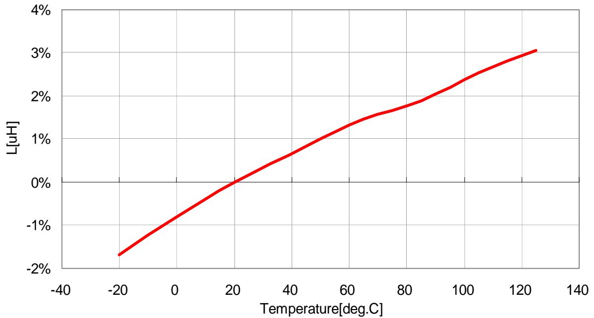
VLF4014ST-6R8M2R2
