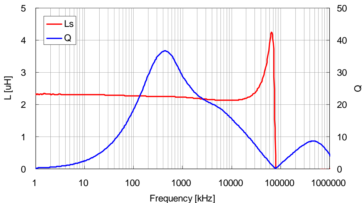
VLF4014ST-2R2M1R9
