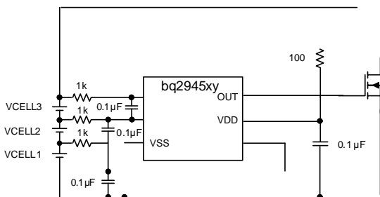
Figure 8. 3-Series Cell Configuration with Fixed Delay
