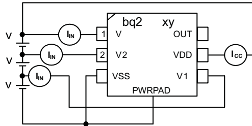
Figure 11. Configuration for IC Current Consumption Test
