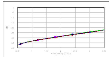
RF3 to RF4 Isolation
